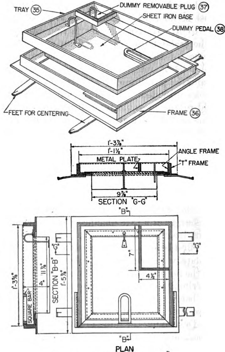
FIGURE 34.—Dummy mine.
